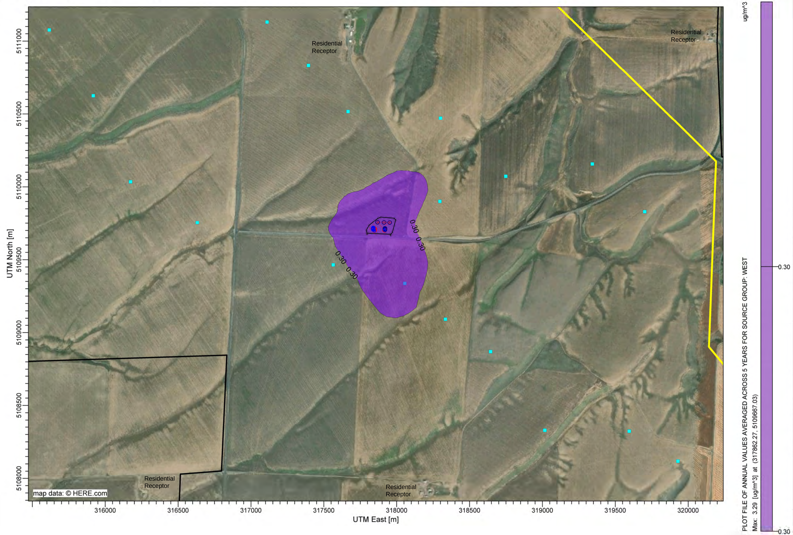
Figure C-9 Horse Heaven - Air Quality Dispersion Modeling Evaluation West Concrete Batch Plant (Phase 2) - Annual PM2.5
