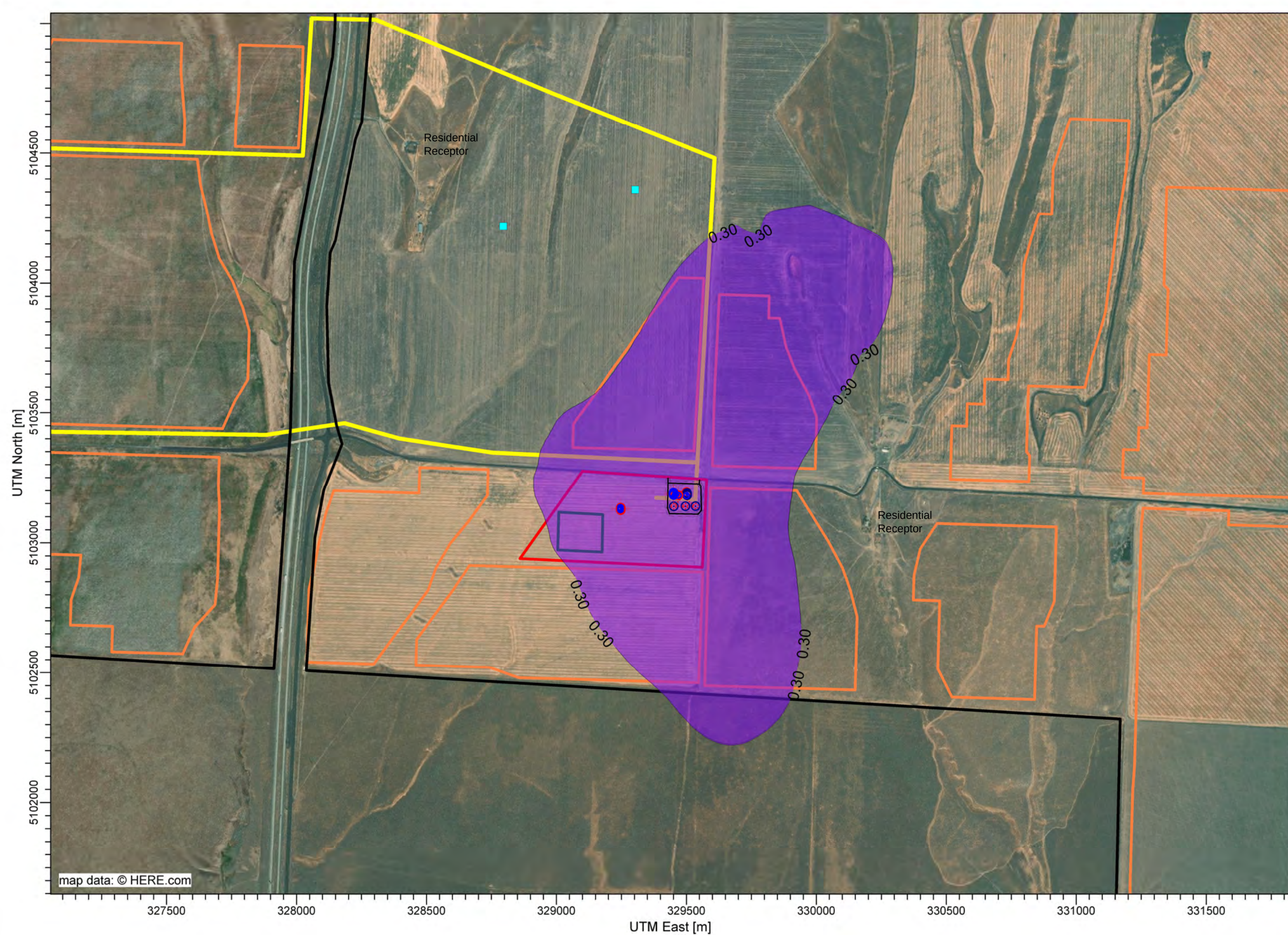
Figure C-8 Horse Heaven - Air Quality Dispersion Modeling Evaluation Stationary Engines and East Concrete Batch Plant (Phase 1) - Annual PM 2.5
