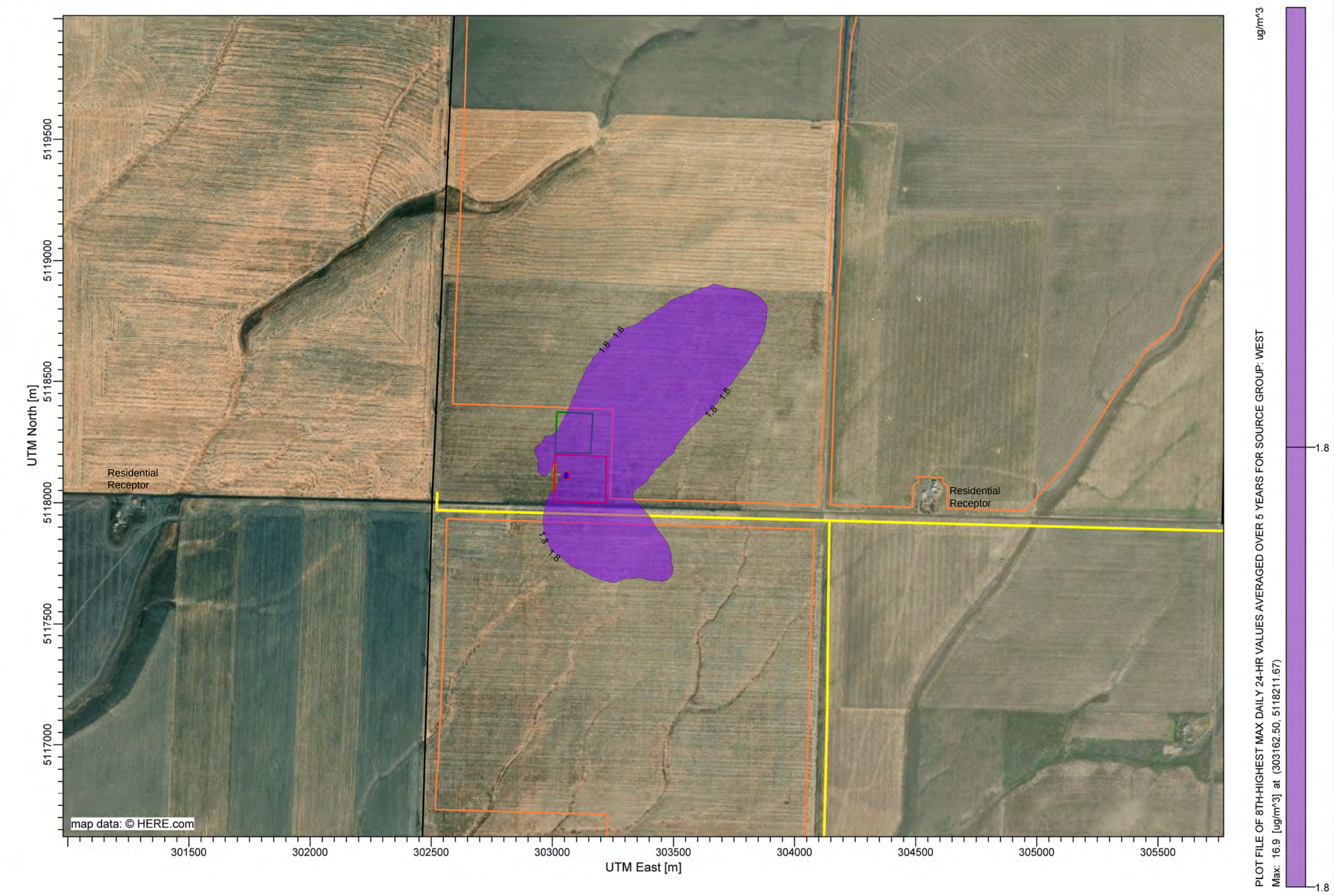
Figure C-5 Horse Heaven - Air Quality Dispersion Modeling Evaluation Stationary Engines - West Substation - 24-hour PM2.5
