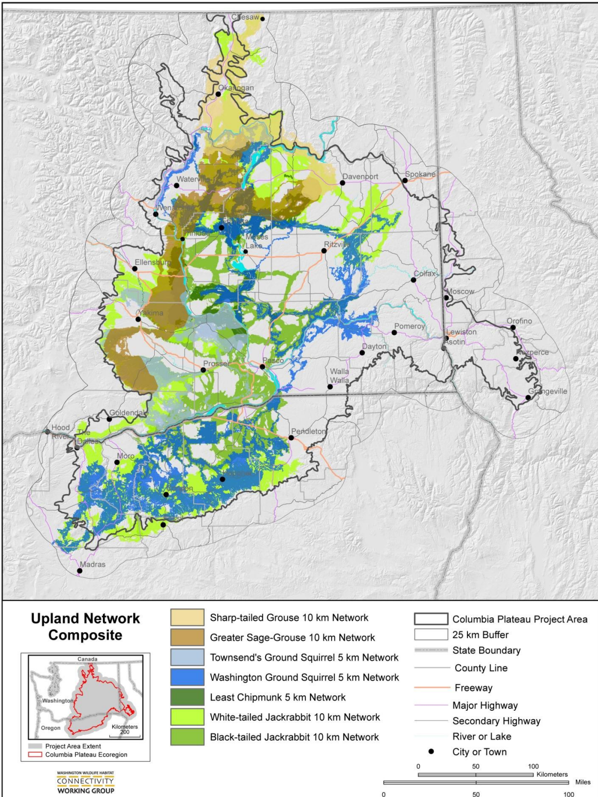
Figure 3.18. Upland Network composite map. This map is based on seven species closely associated with upland shrubsteppe habitat.
